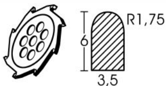
Carbide blade Ø 110 x 3.5 mm, round
